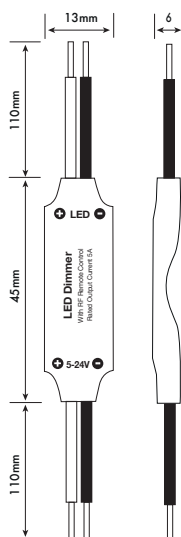
LED Dimmer Unit
