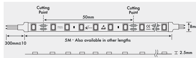
120 LEDs per metre | Single colour
