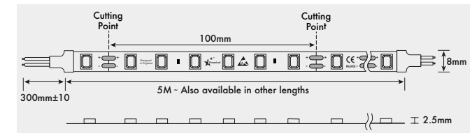
60 LEDs per metre | Single colour
