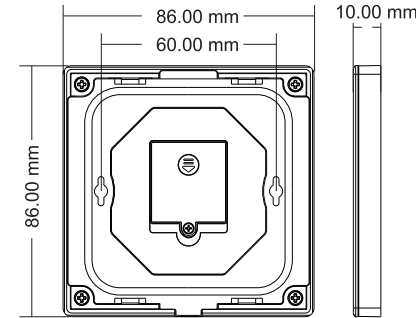
Installation diagram:
